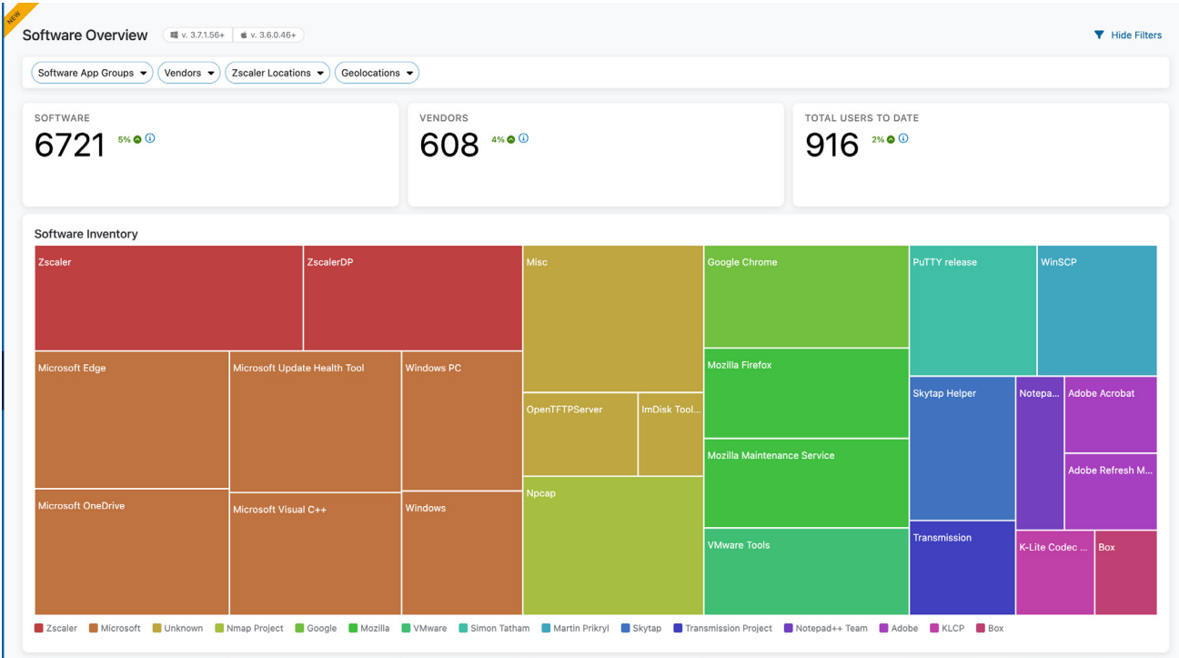
Figure 27: The Software Inventory page with applications grouped by vendor and scaled by user count, with hover-over details showing the number of versions and users
