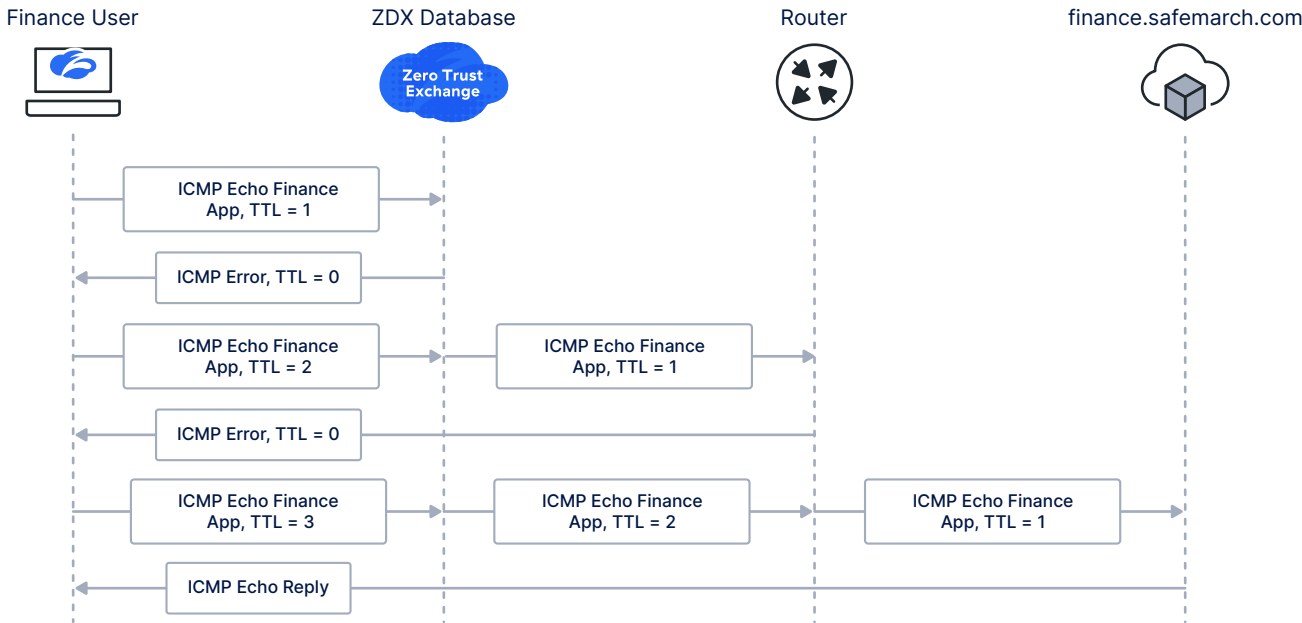
Figure 7: Cloud Path probes send requests with incremental TTL settings to probe each hop in the network path
