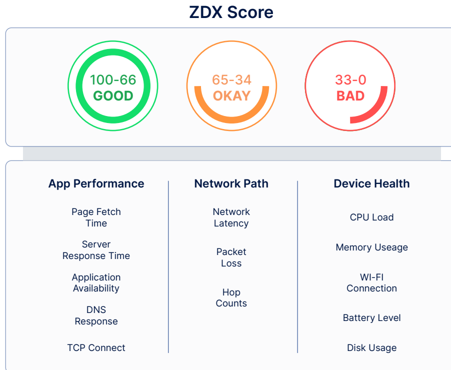
Figure 14: The ZDX Score takes in multiple inputs and reports at the organization, region, site, and user level
