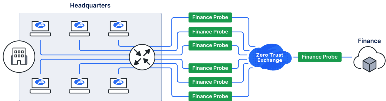
Figure 8: Smart caching prevents applications from being flooded with probe requests
