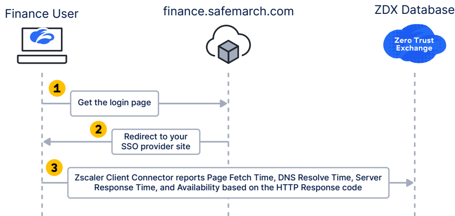
Figure 6: Web probes send HTTP/HTTPS GET requests to your application and monitor the HTTP Status Code that is returned
