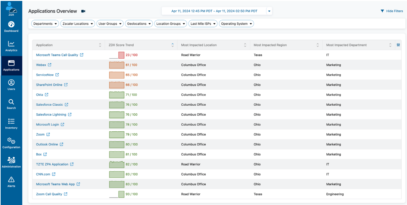
Figure 16: The ZDX Applications Overview dashboard
