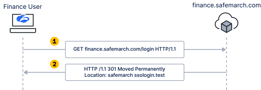
Figure 12: It's important that you monitor the correct service and response codes
