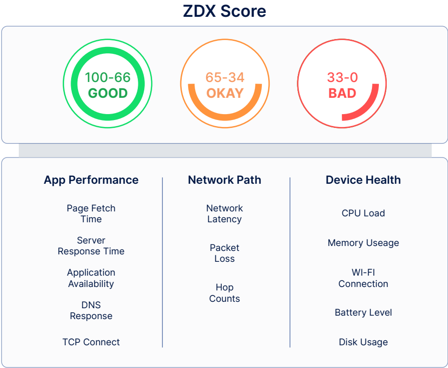
Figure 1: Digital experience monitoring provides end-to-end visibility from the user's perspective
