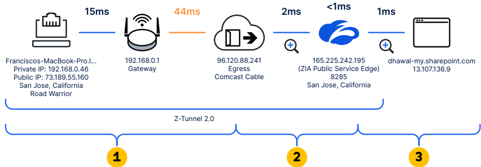
Figure 41: Defined segment groups in the ZIA path
