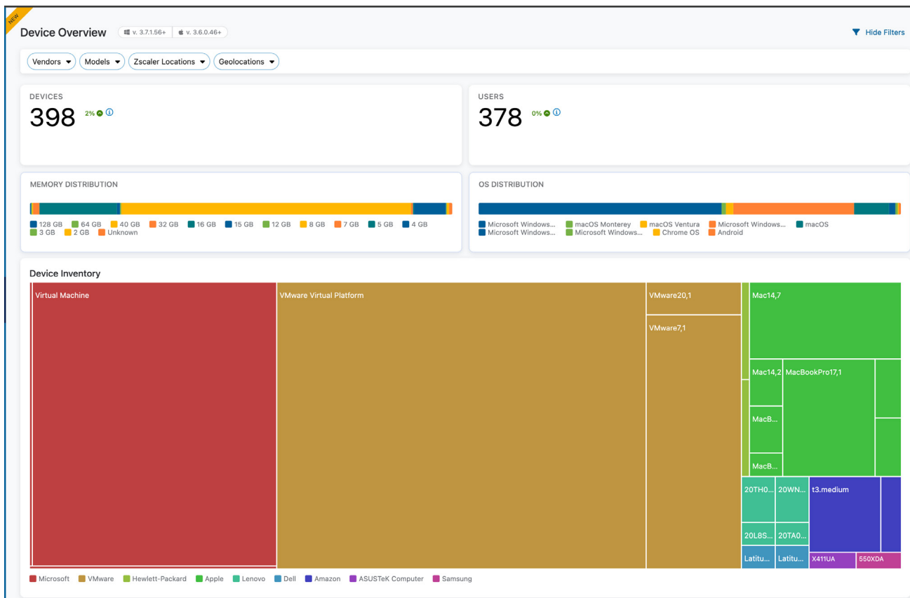
Figure 28: The Device Overview page with applications grouped by vendor and scaled by user count
