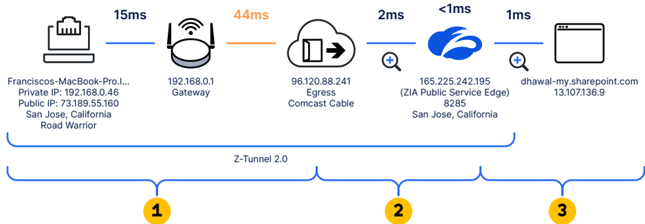
Figure 24: Hop view gives you details about the path from your user to an application
