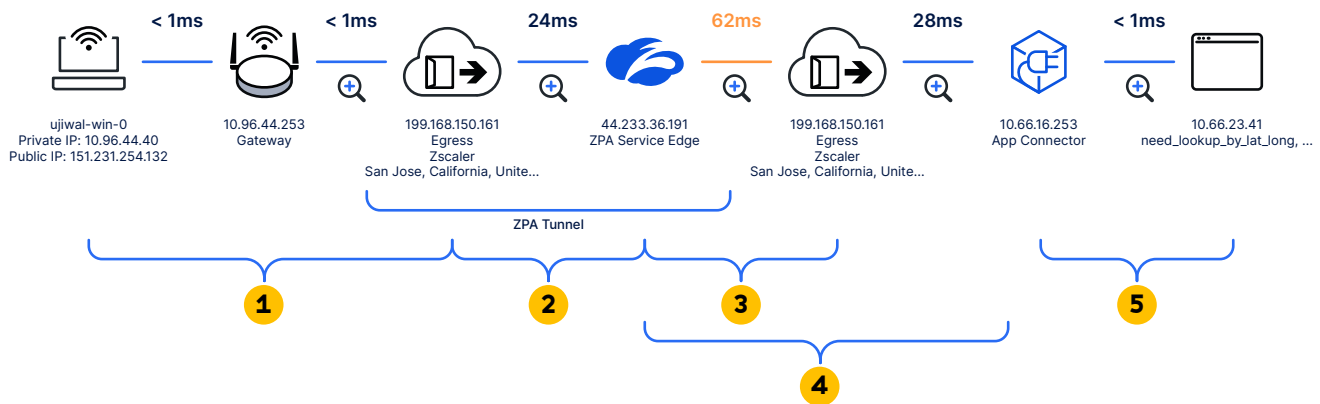
Figure 41: Defined segment groups in the ZPA path
