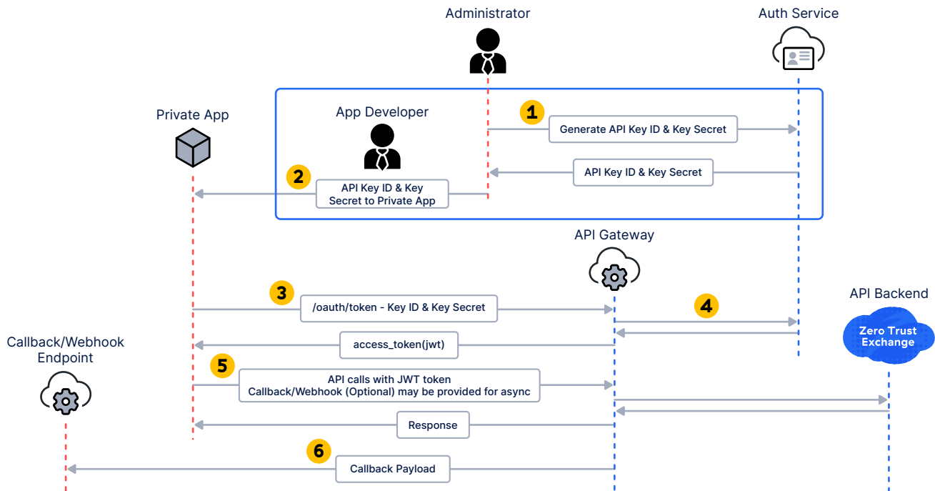
Figure 40: The ZDX API access flow
