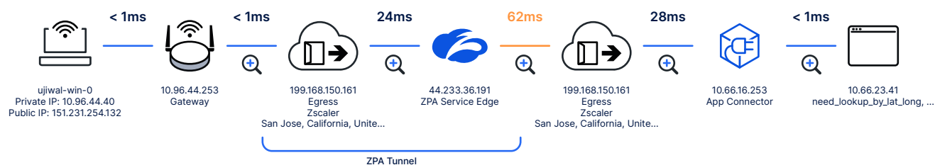
Figure 2: ZDX gives you visibility into your device and the network between your user and the application they are using
