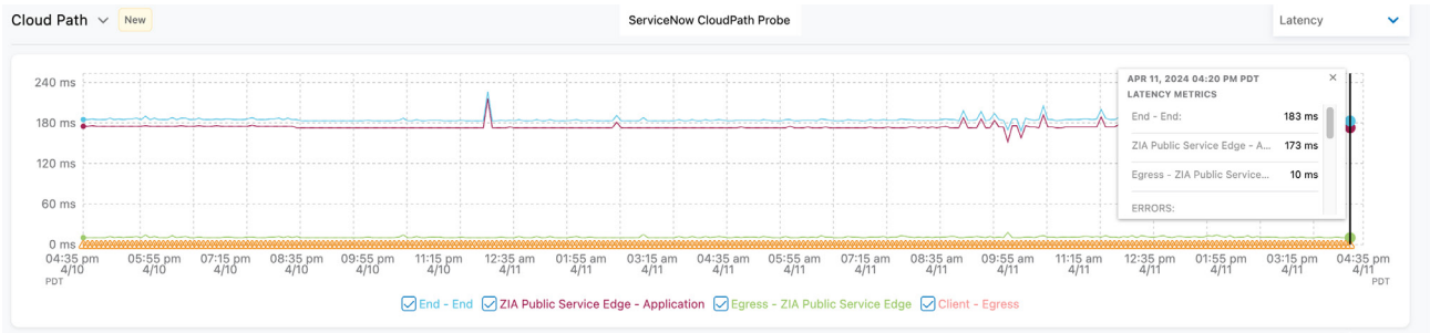
Figure 23: Cloud Path metrics over time
