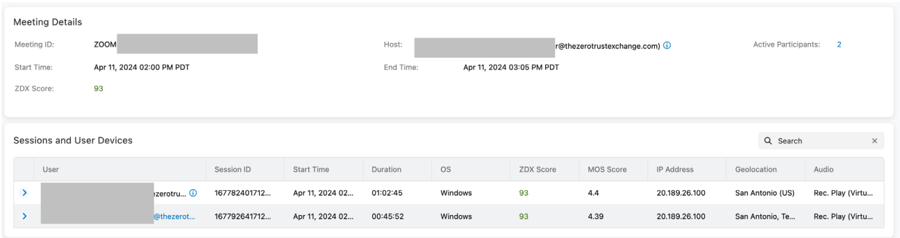
Figure 36: Meeting details allow you to quickly scan key metrics related to meeting quality
